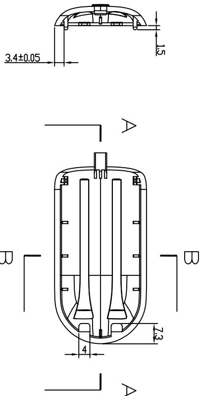
SECTION B—B
